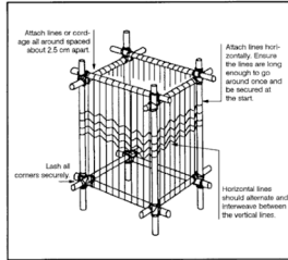
Figure 12-10. Square pack.
