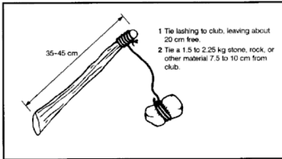
Figure 12-2. Sling club.
