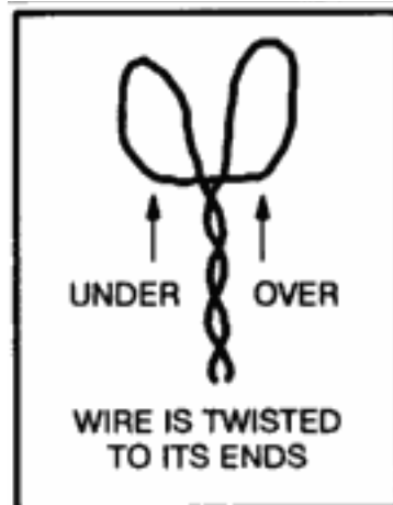
DOUBLE WIRE LOCKING LOOP
